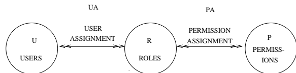
Figure 1: Flat RBAC
